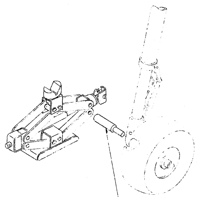
200-590016-003 PAD-MAIN WHEEL
